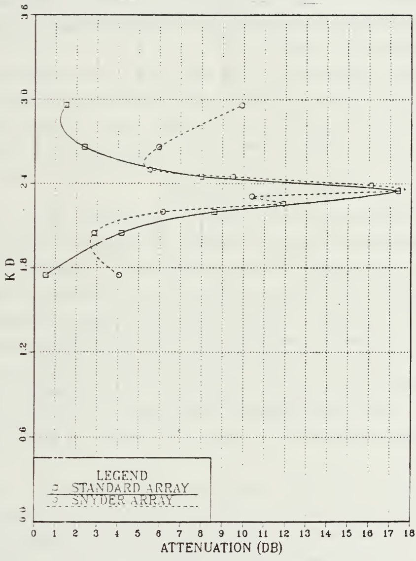
Figure 4.19 Attenuation Comparison.
