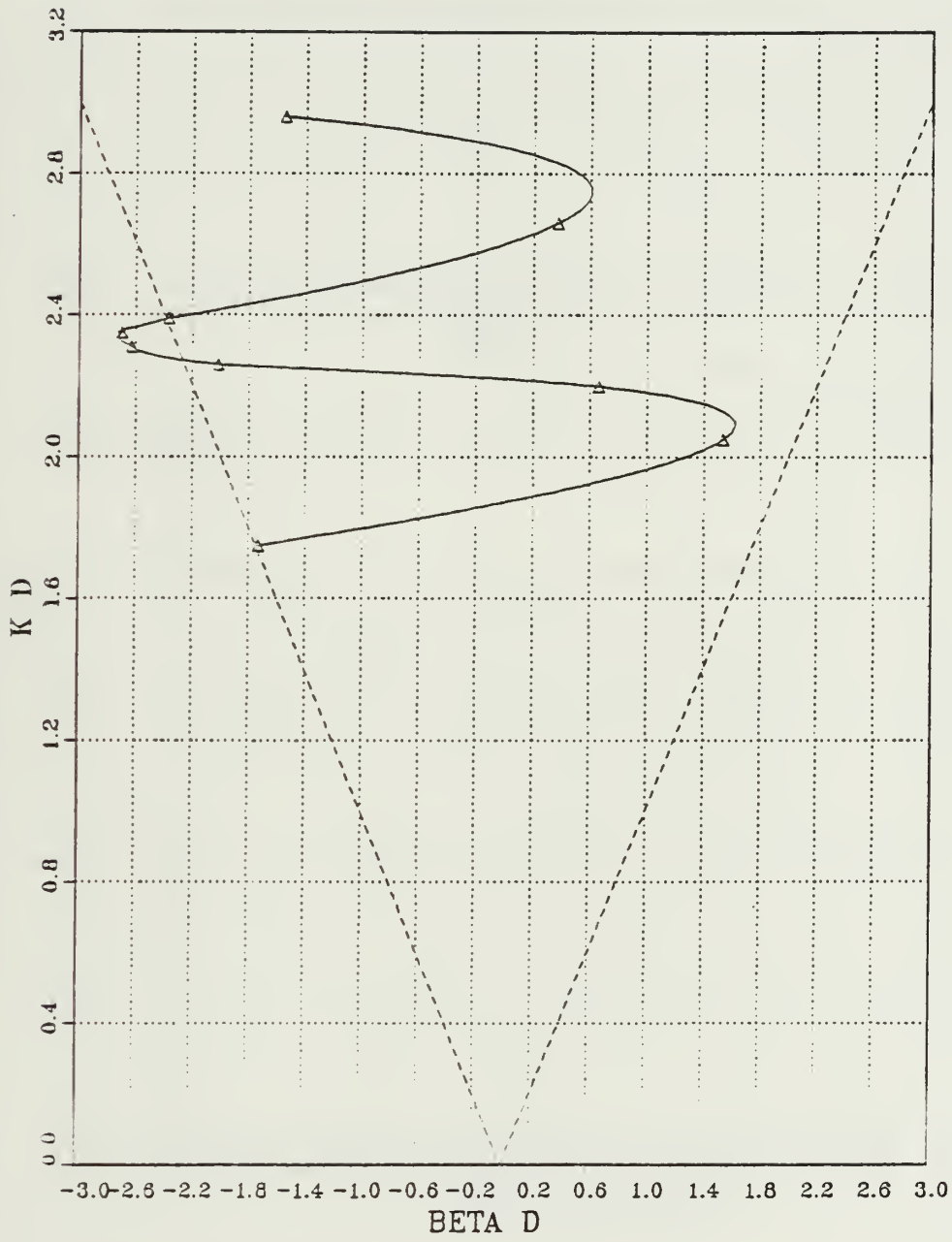
Figure 4.12 k-β Diagram for a Snyder Switched Parallel Array. Element Spacing = 3/8 Wavelength.
